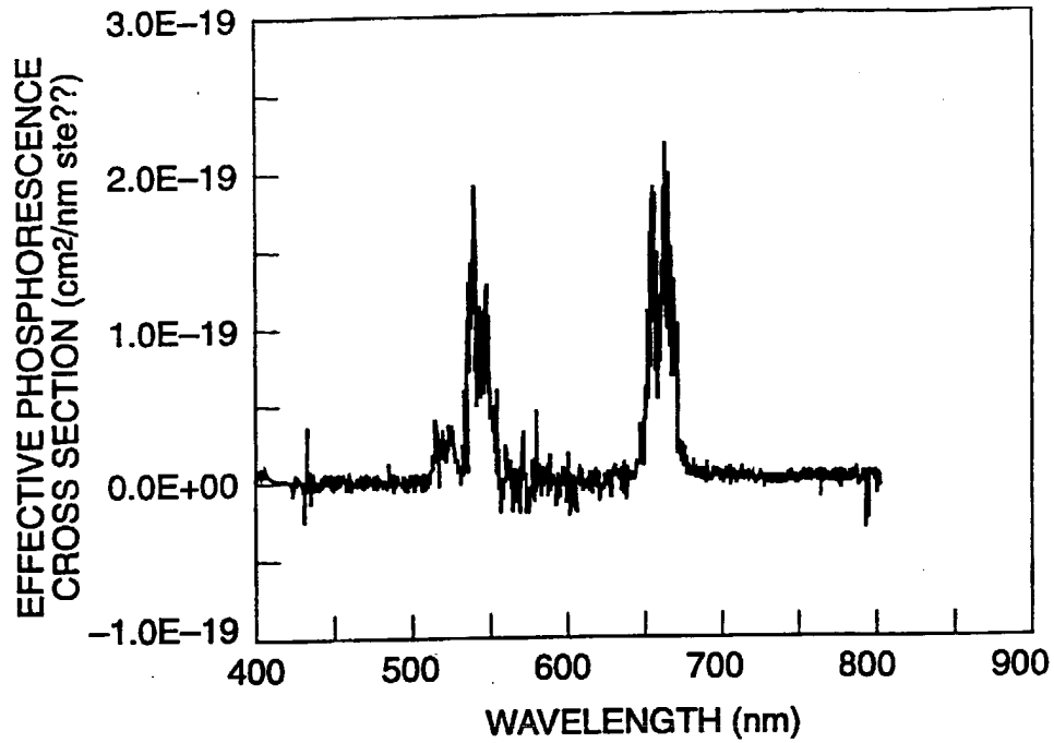
PHOSPHORESCENCE FOR Na(Y 0.8 Yb 0.18 Er 0.02 )F 4 , - 975 nm PUMP
